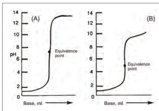
Figure 1: Curves show difference between strong acid (A) titrated with strong base, and (B) titrated with a weak base.
